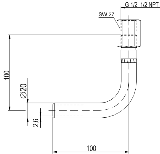
Elbow 90°
